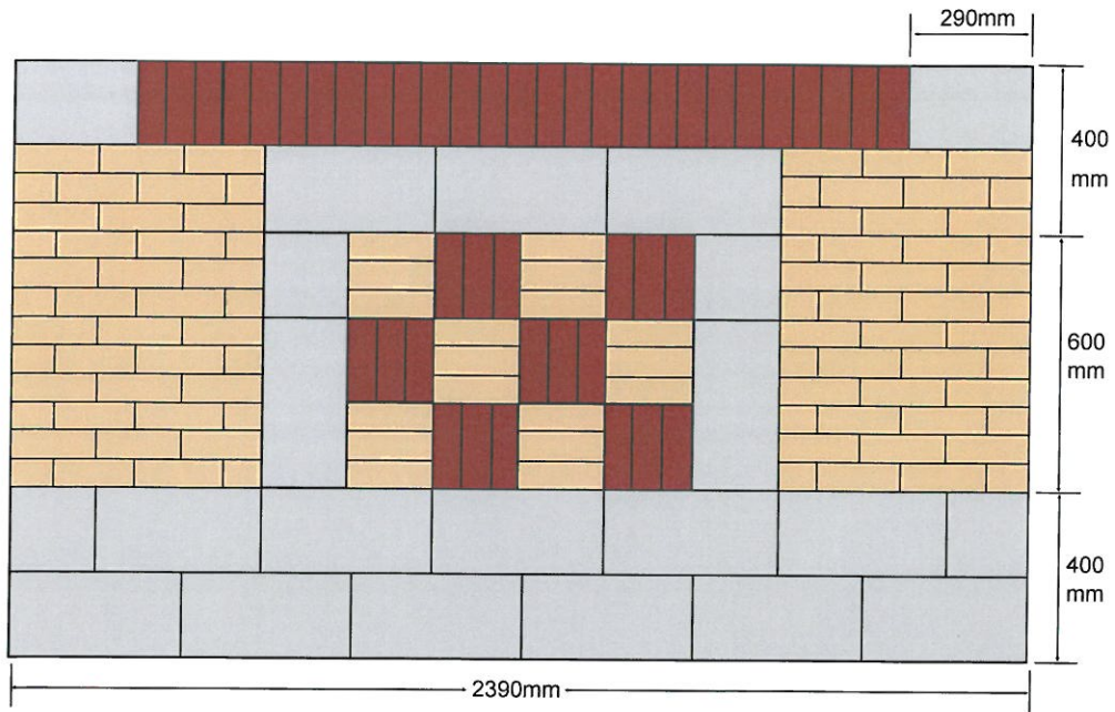
Front elevation Elevation avant
